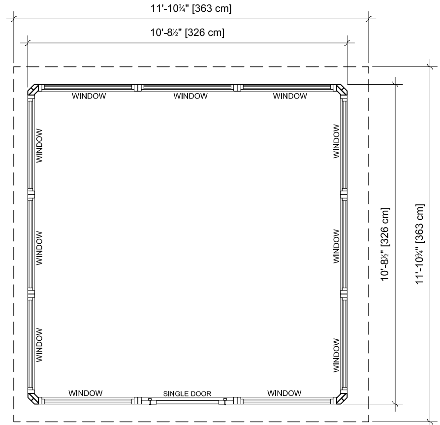
Footprint Plan
